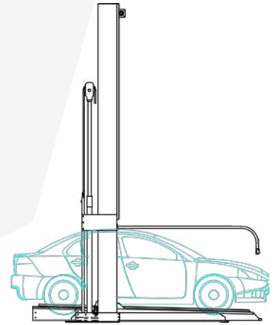
» System lowered
